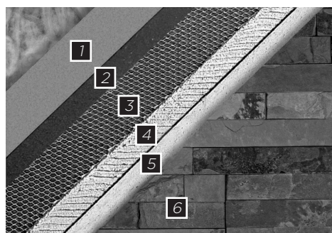
[1] Rigid foam insulation, [2] SM-BT, [3] Lath, [4] Mortar/scratch coat, [5] Mortar setting bed, [6] TerraCraft®
