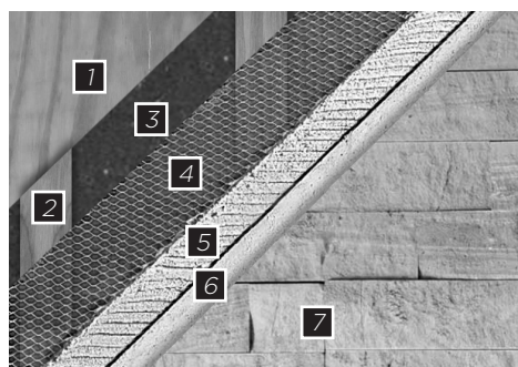
[1] Sheathing, [2] 10mm P.T. wood strapping, [3] SM-BT, [4] Lath, [5] Mortar/scratch coat, [6] Mortar setting bed, [7] TerraCraft®
