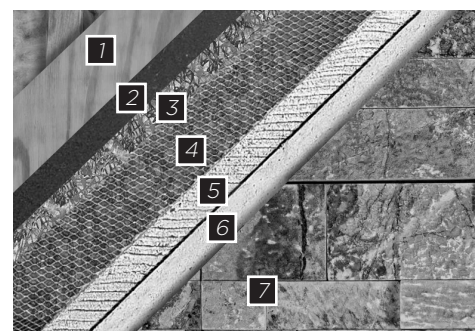
[1] Sheathing, [2] SM-BT, [3] Drainage mat, [4] Lath, [5] Mortar/scratch coat, [6] Mortar setting bed, [7] TerraCraft®
