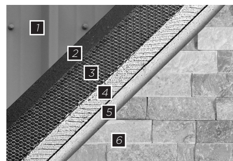
[1] Metal building, [2] SM-BT, [3] Lath, [4] Mortar/scratch coat, [5] Mortar setting bed, [6] TerraCraft®
