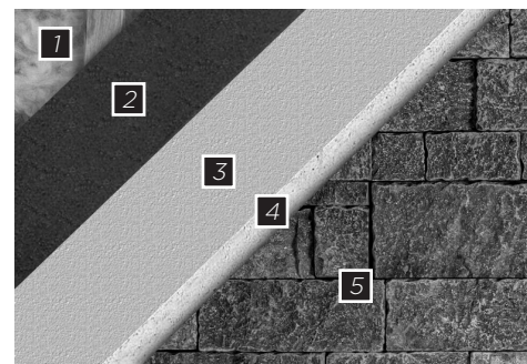
[1] Wood or steel studs, [2] SM-BT, [3] Cement board, [4] Mortar setting bed*, [5] TerraCraft®
